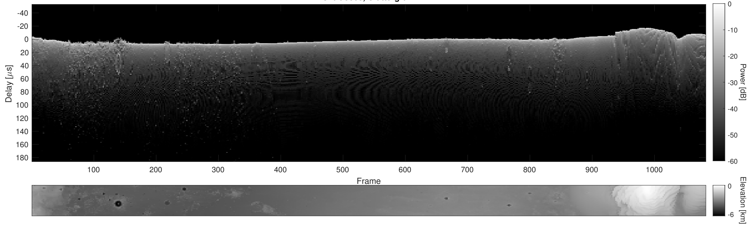
Orbit 5868, Cluttergram
