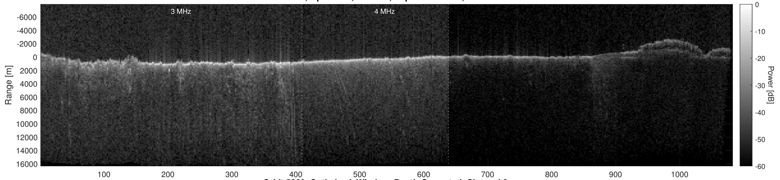
Orbit 5868, Optimized, Window, Depth-Corrected, Channel 2
