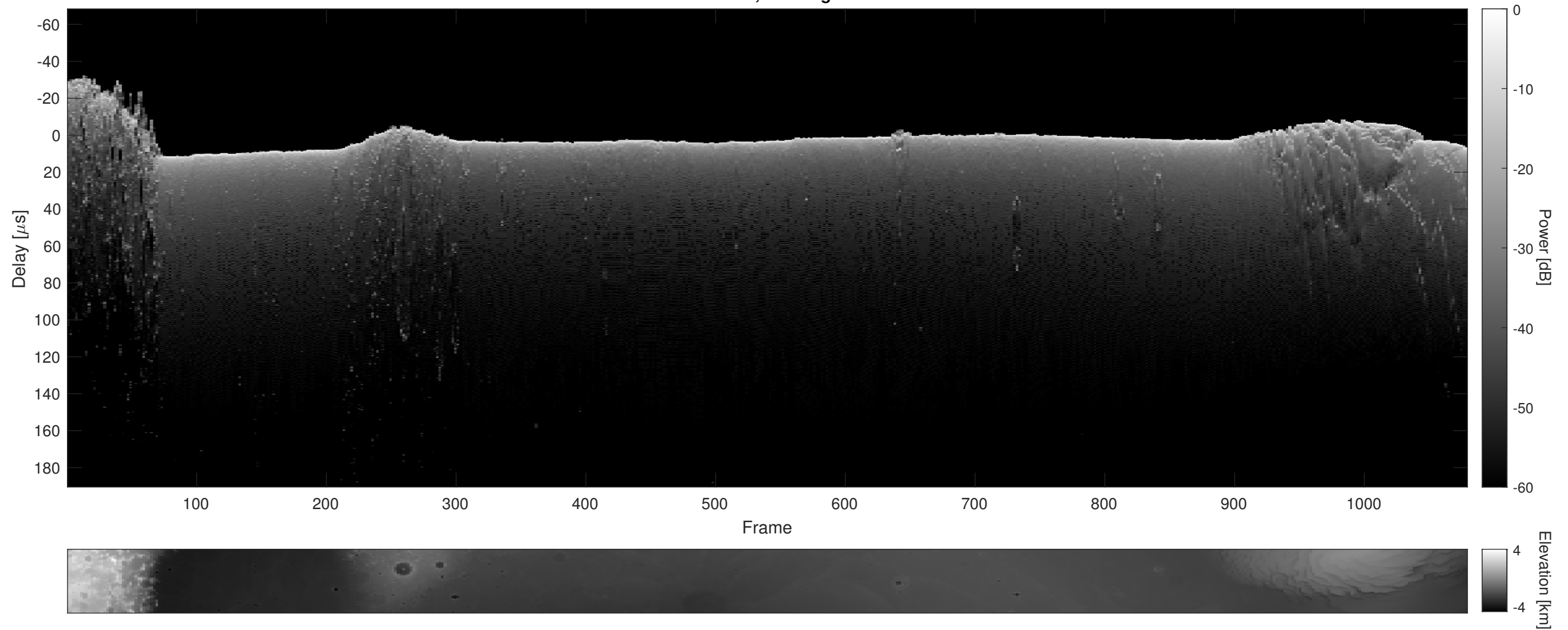
Orbit 5869, Cluttergram
