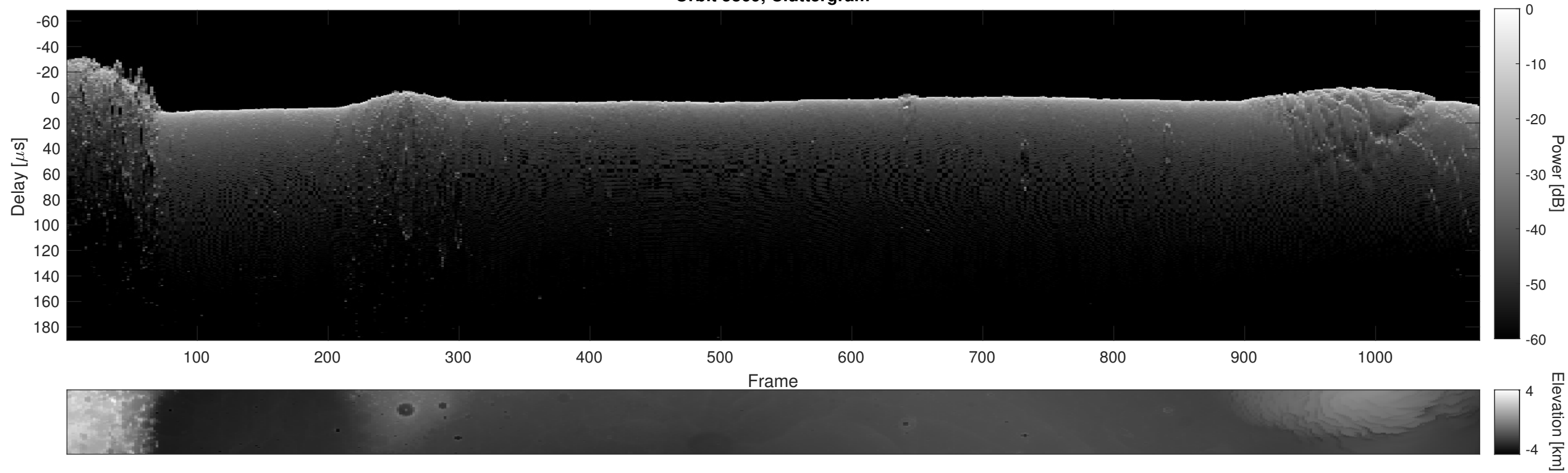
Orbit 5869, Cluttergram
