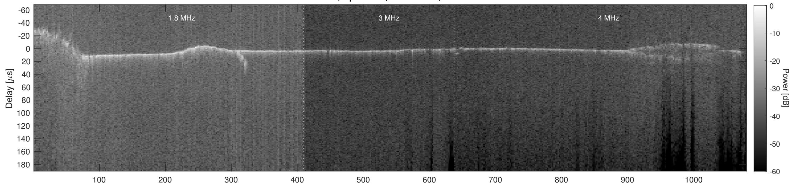
Orbit 5869, Cluttergram
