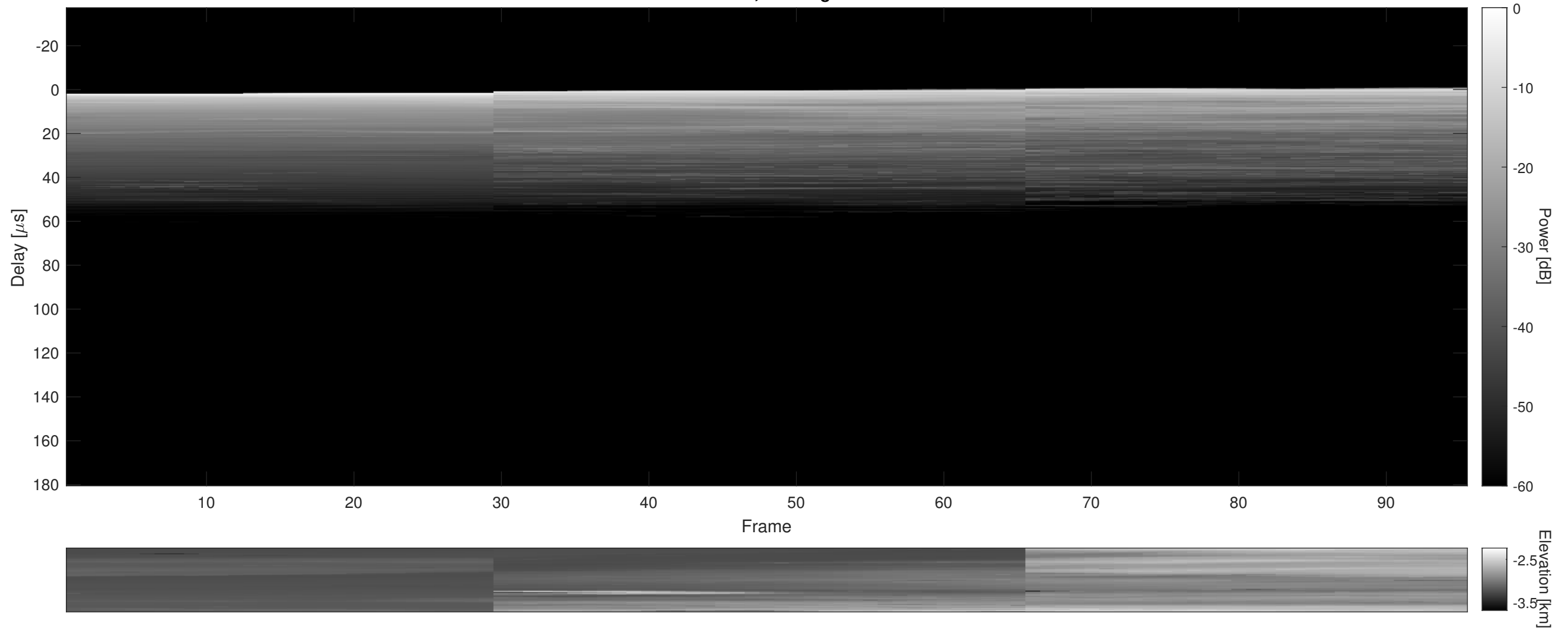
Orbit 5870, Cluttergram
