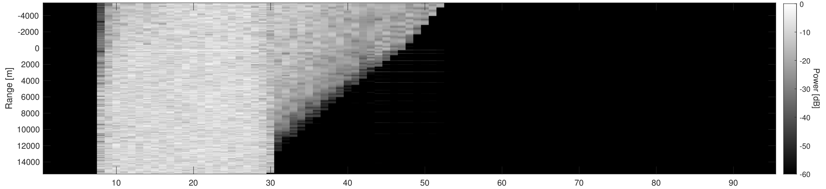
Orbit 5870, Depth-Corrected Cluttergram
