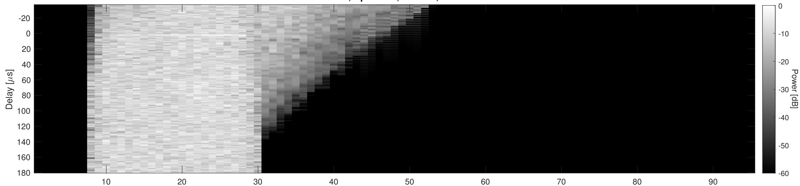
Orbit 5870, Cluttergram
