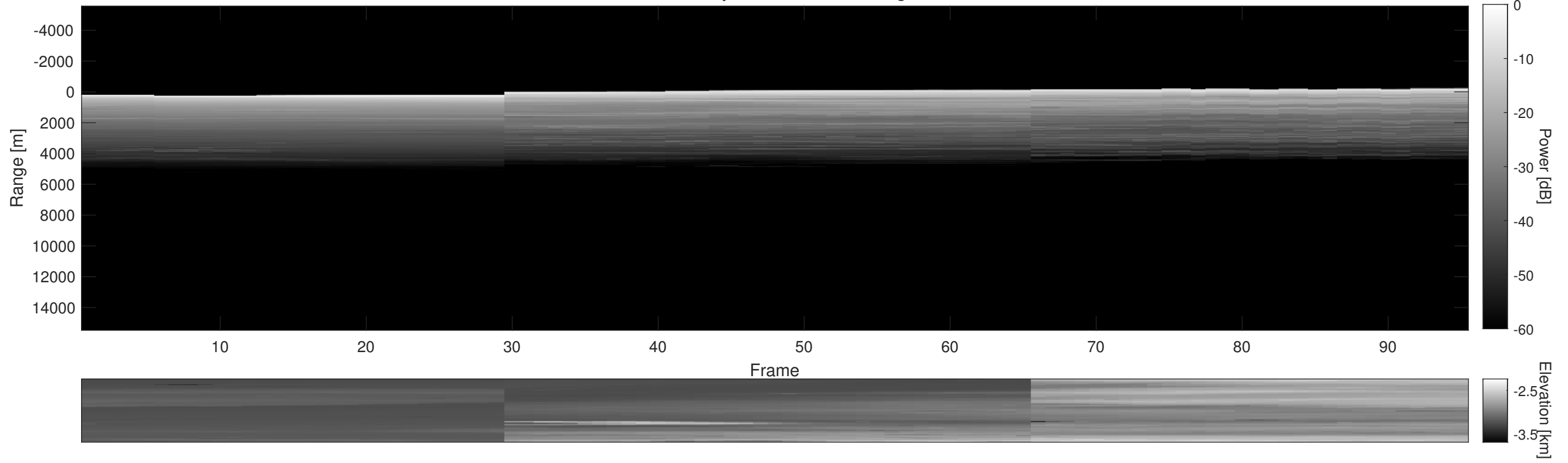
Orbit 5870, Depth-Corrected Cluttergram
