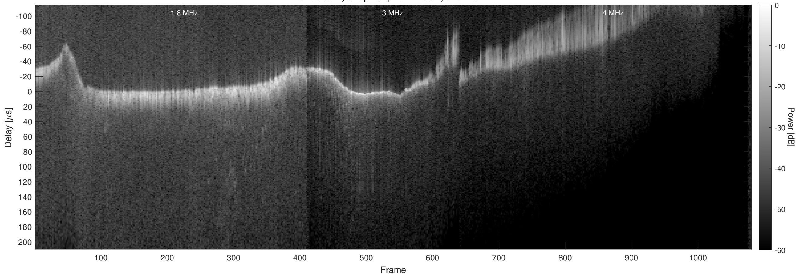
Orbit 5871, Chapman, No Window, Channel 2
