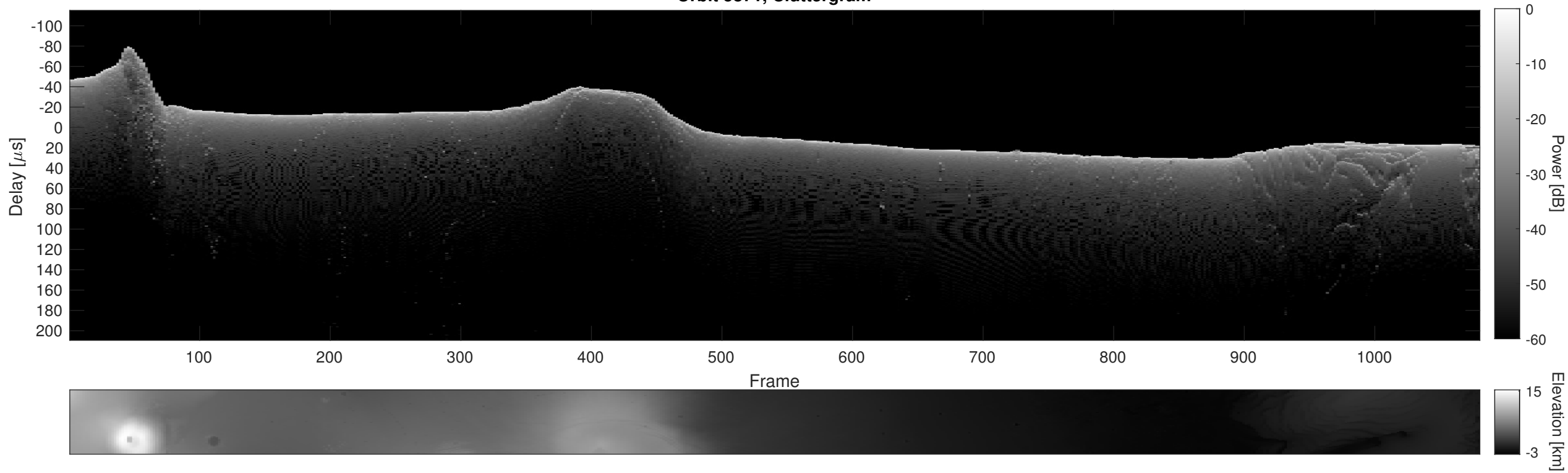
Orbit 5871, Cluttergram
