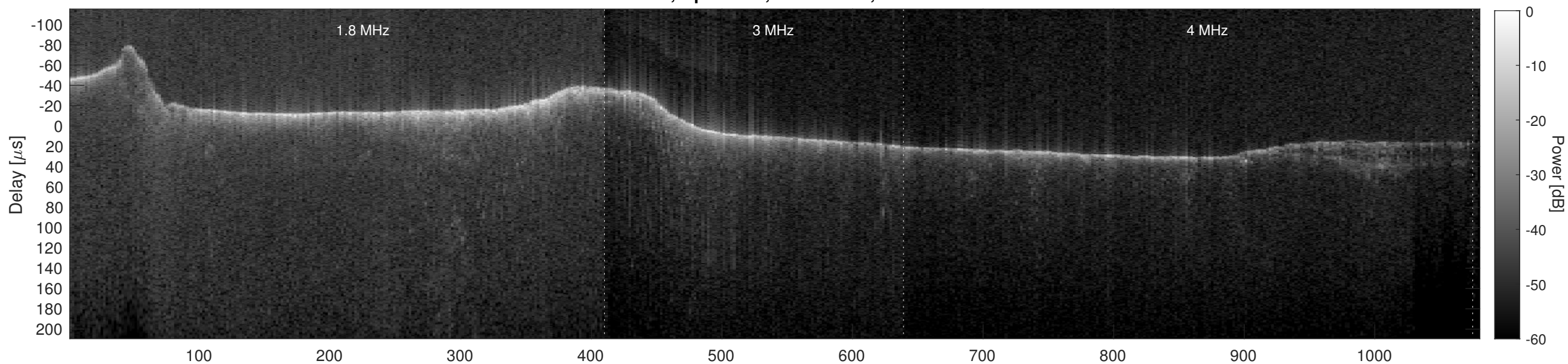
Orbit 5871, Cluttergram
