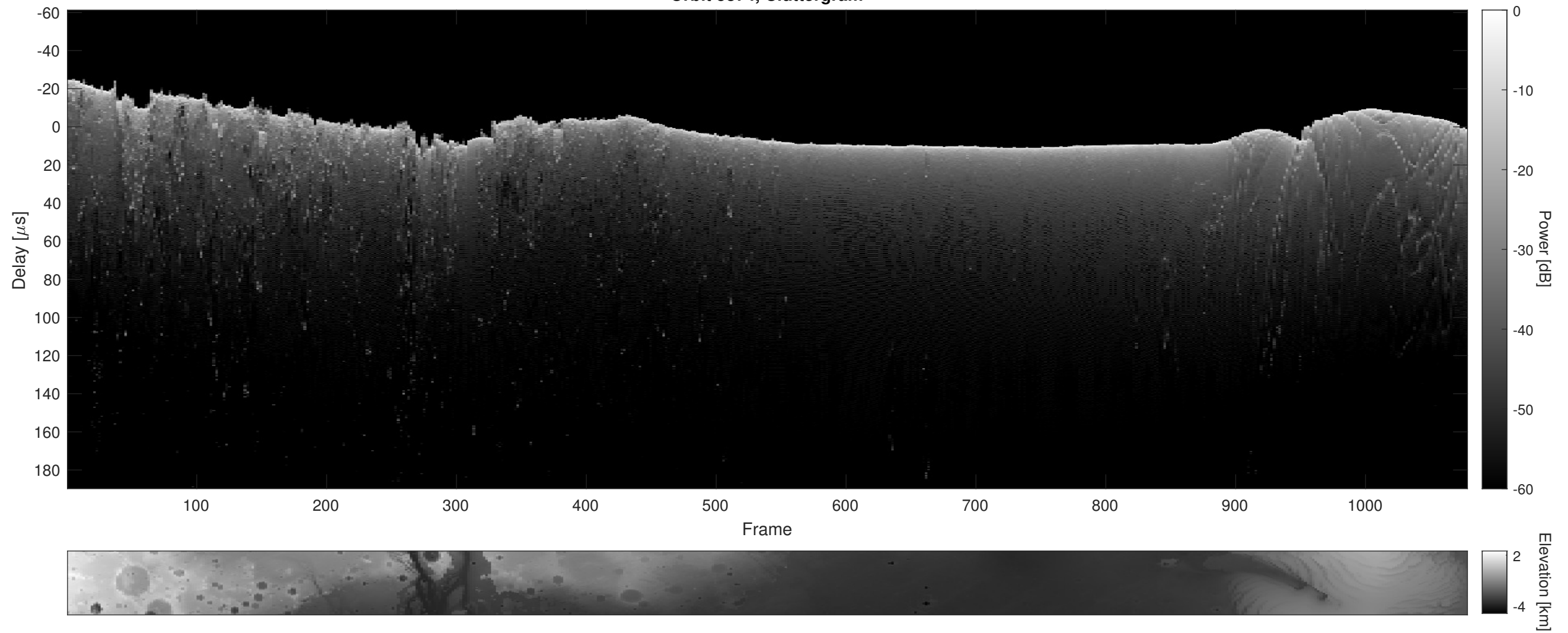
Orbit 5874, Cluttergram
