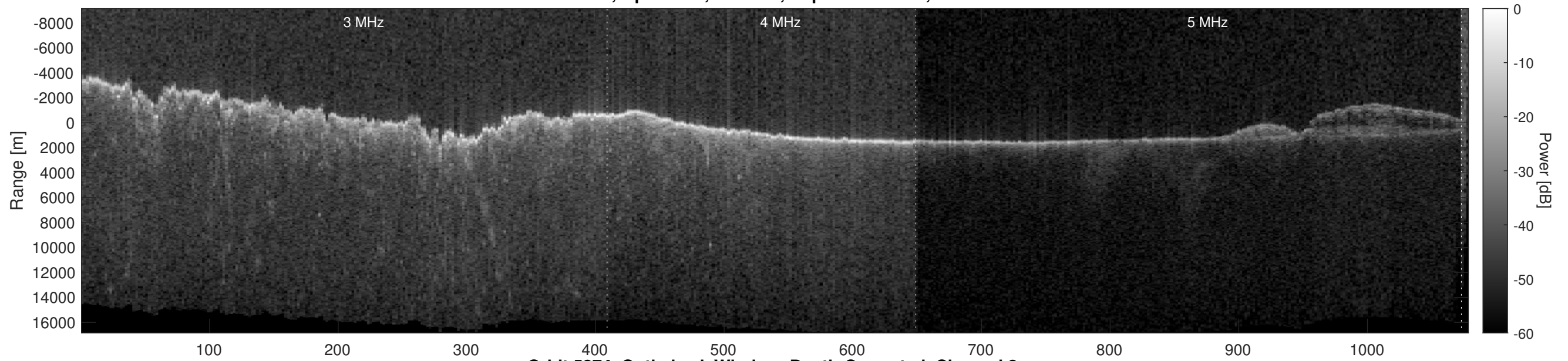
Orbit 5874, Optimized, Window, Depth-Corrected, Channel 2
