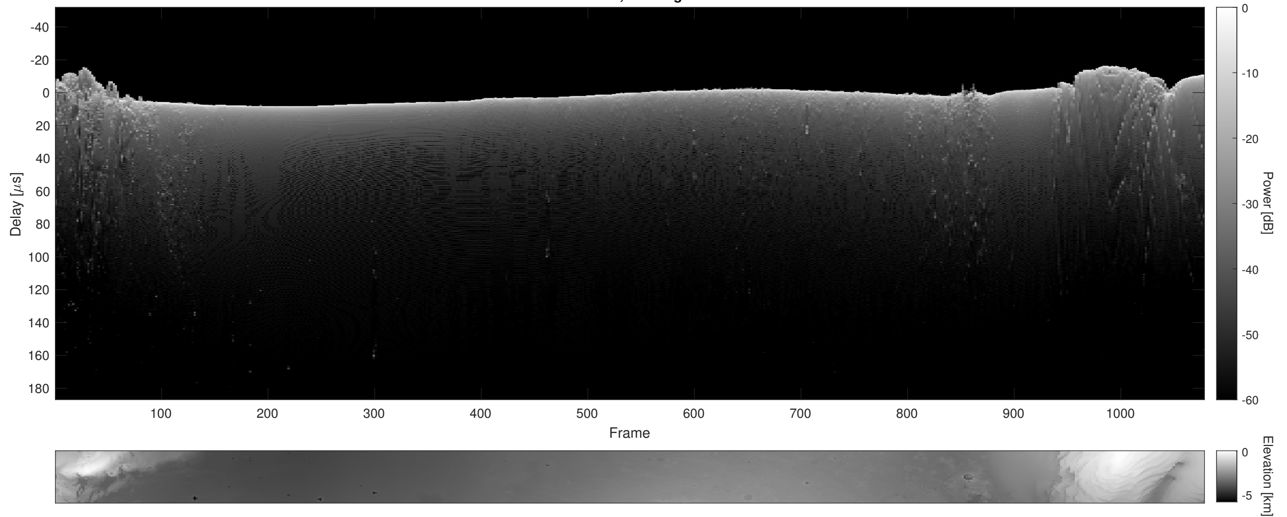
Orbit 5875, Cluttergram
