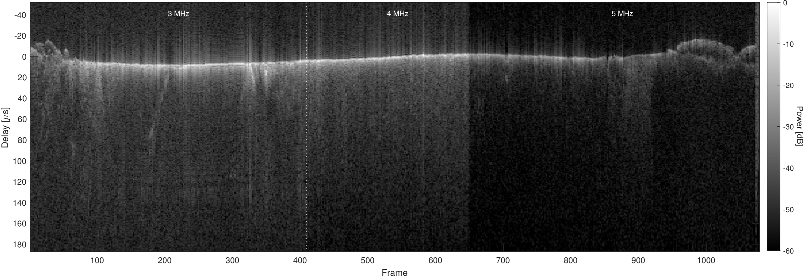
Orbit 5875, Optimized, No Window, Channel 2
