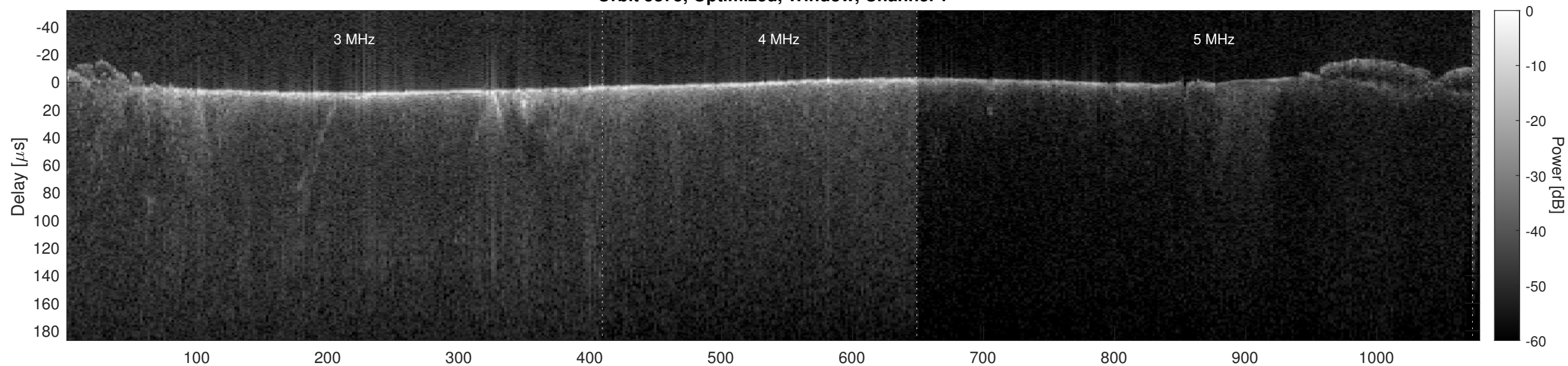
Orbit 5875, Optimized, Window, Channel 2
