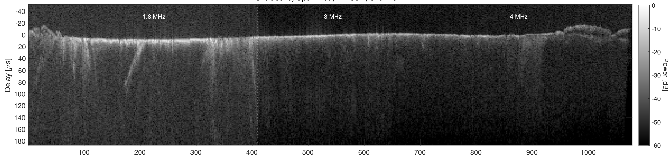
Orbit 5875, Cluttergram
