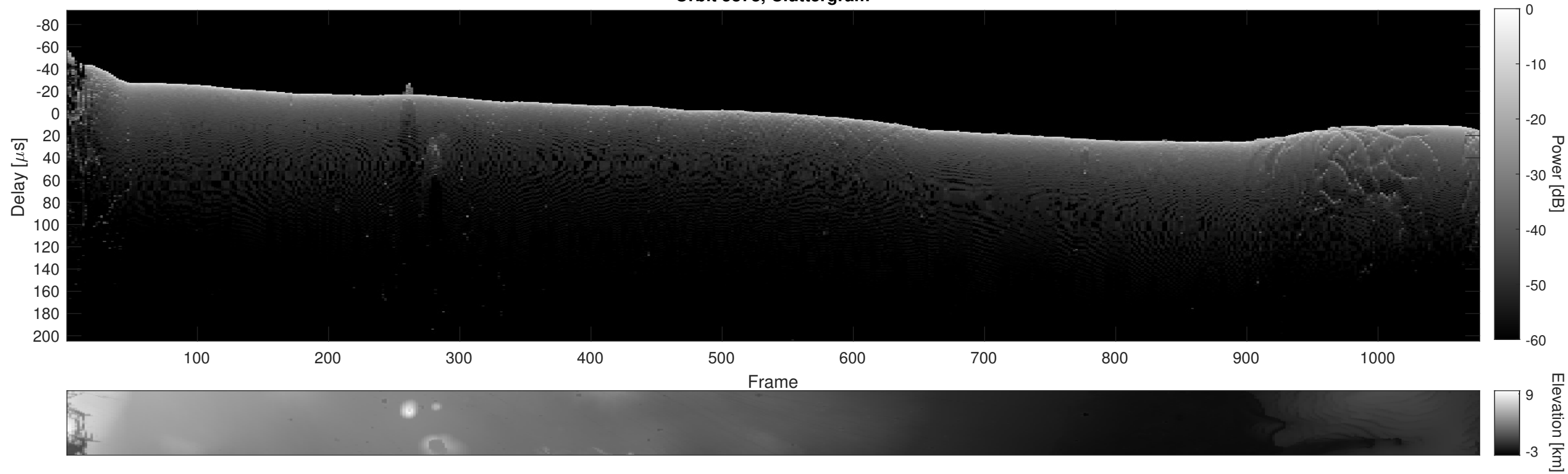
Orbit 5878, Cluttergram
