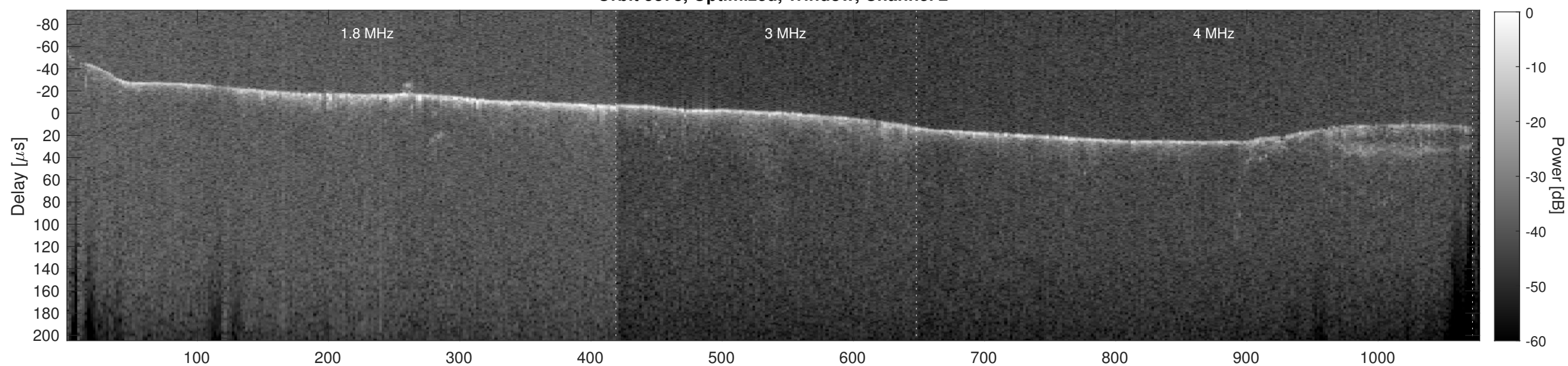
Orbit 5878, Cluttergram
