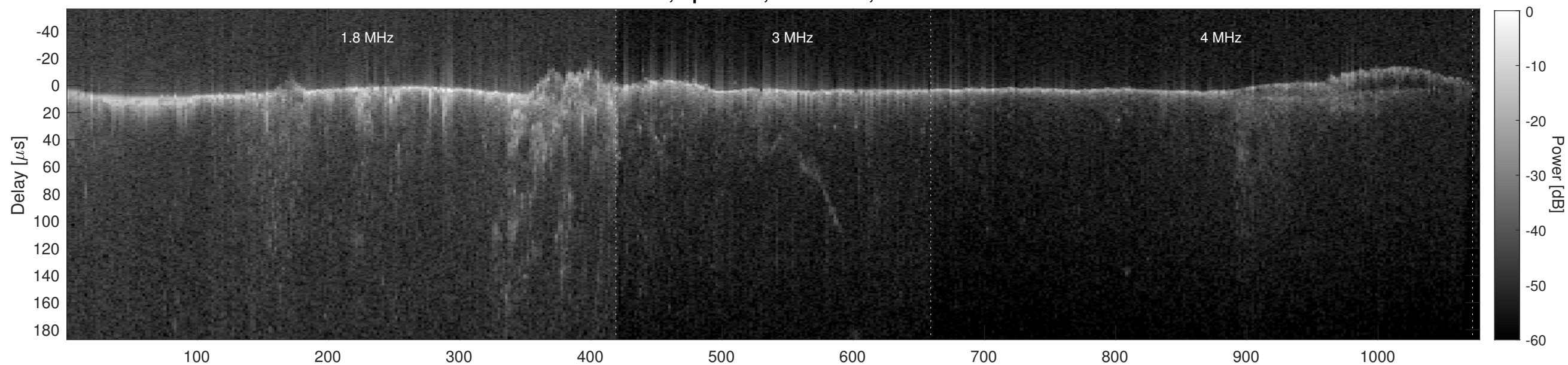
Orbit 5879, Cluttergram
