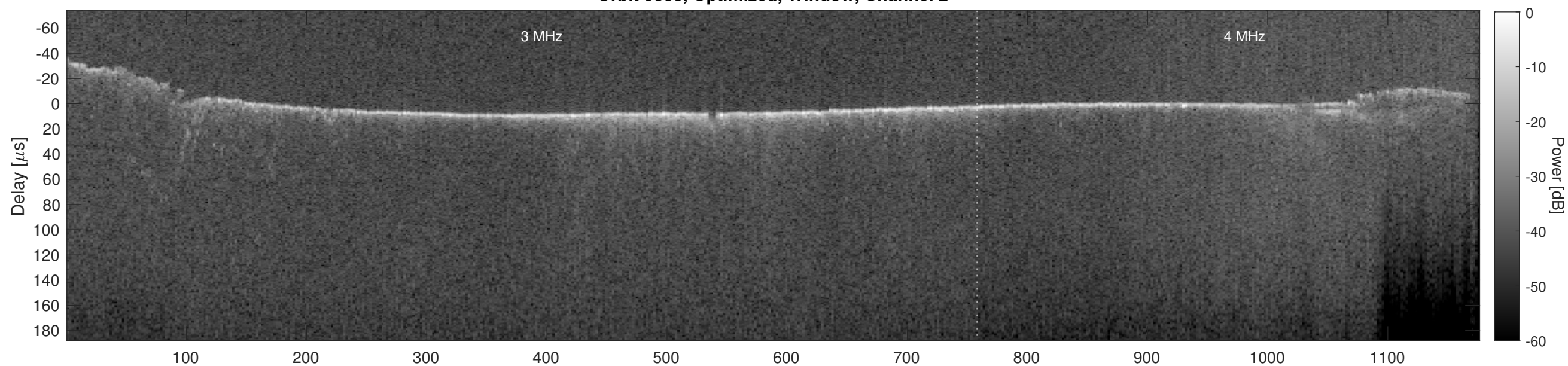
Orbit 5883, Cluttergram
