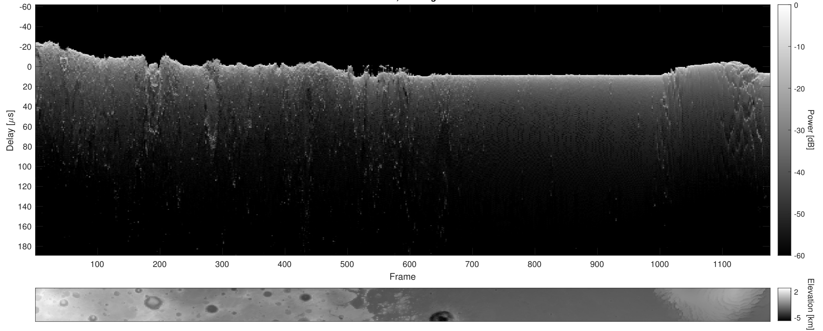
Orbit 5884, Cluttergram
