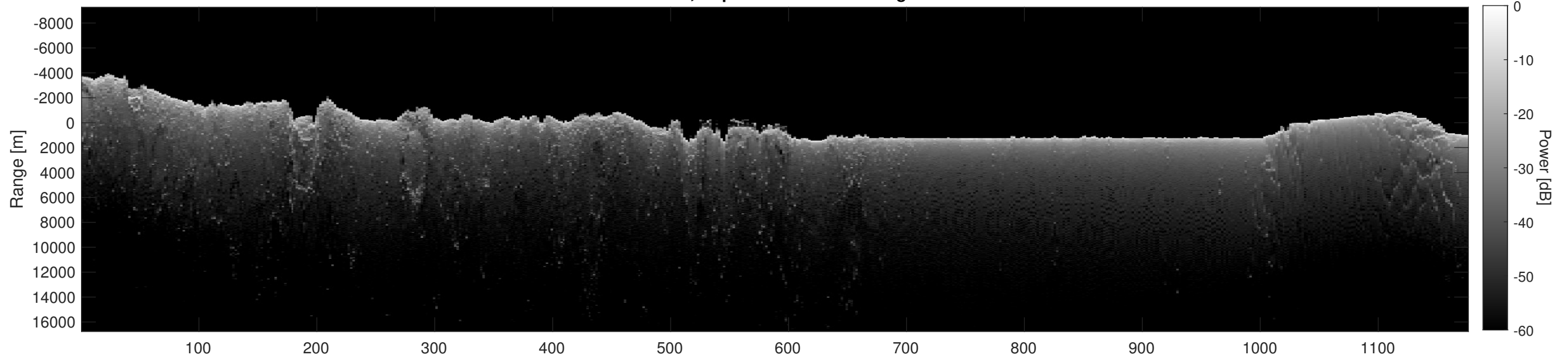
Orbit 5884, Depth-Corrected Cluttergram
