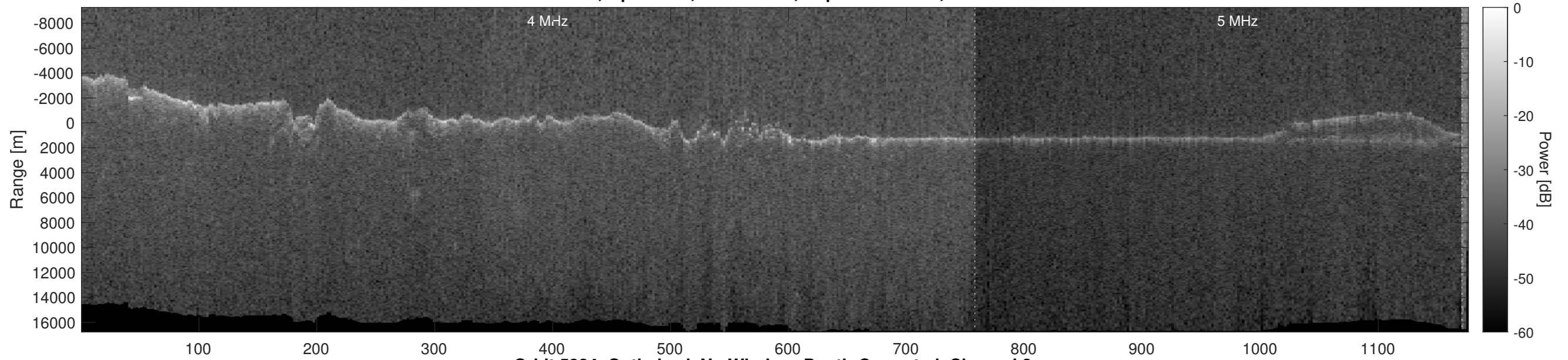
Orbit 5884, Optimized, No Window, Depth-Corrected, Channel 2
