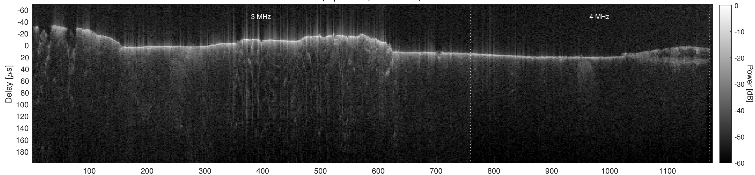
Orbit 5885, Cluttergram
