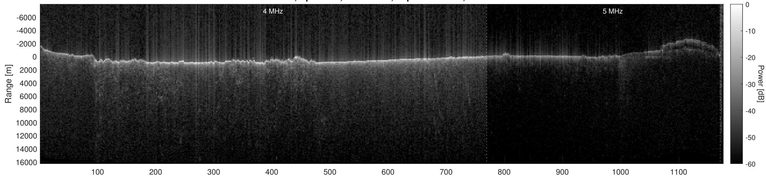
Orbit 5886, Optimized, No Window, Depth-Corrected, Channel 2
