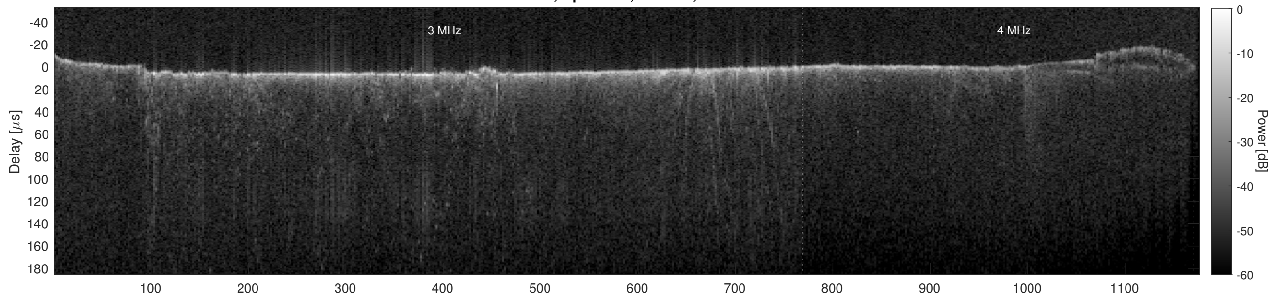
Orbit 5886, Cluttergram
