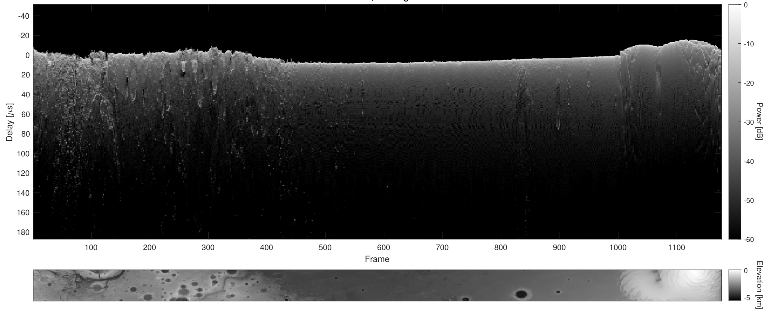
Orbit 5888, Cluttergram
