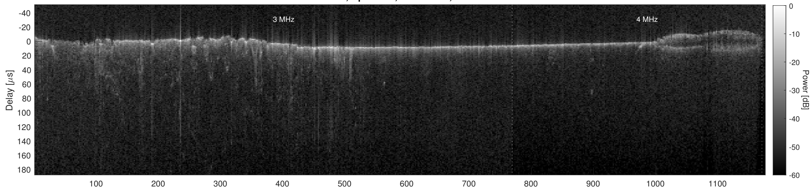
Orbit 5888, Cluttergram
