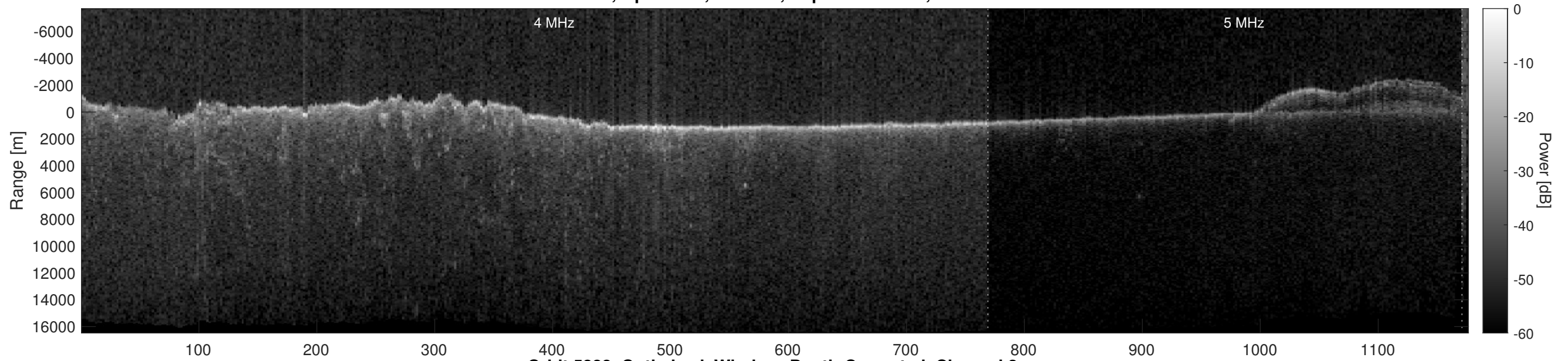
Orbit 5888, Optimized, Window, Depth-Corrected, Channel 2
