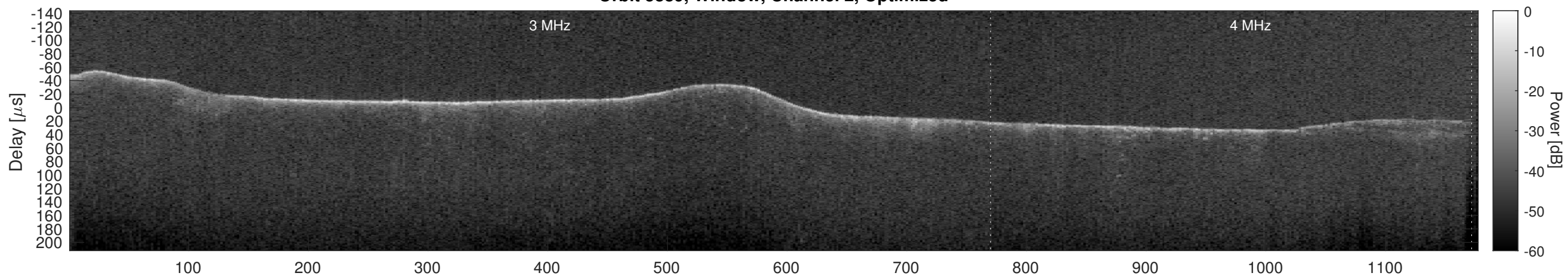
Orbit 5889, Cluttergram
