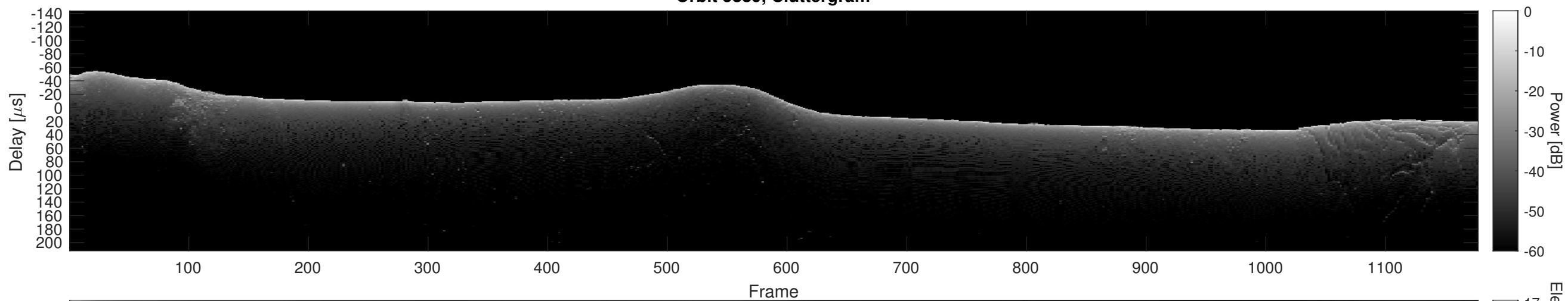
Orbit 5889, Cluttergram
