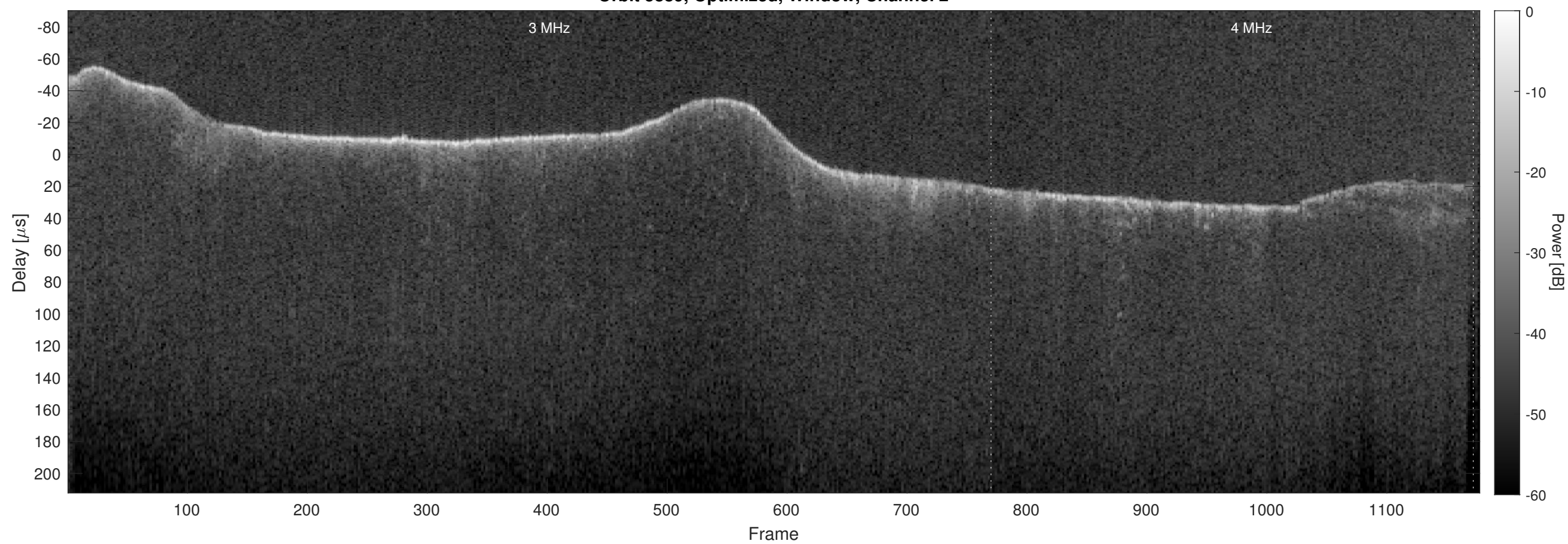
Orbit 5889, Optimized, Window, Channel 2
