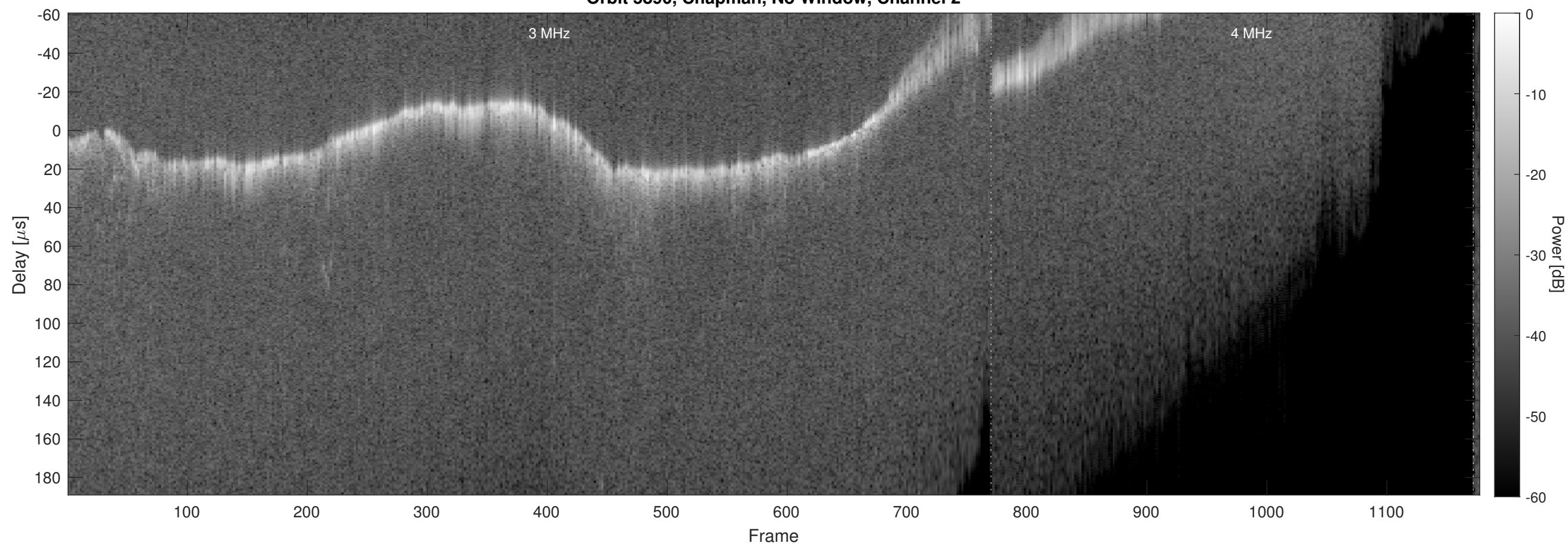
Orbit 5890, Chapman, No Window, Channel 2
