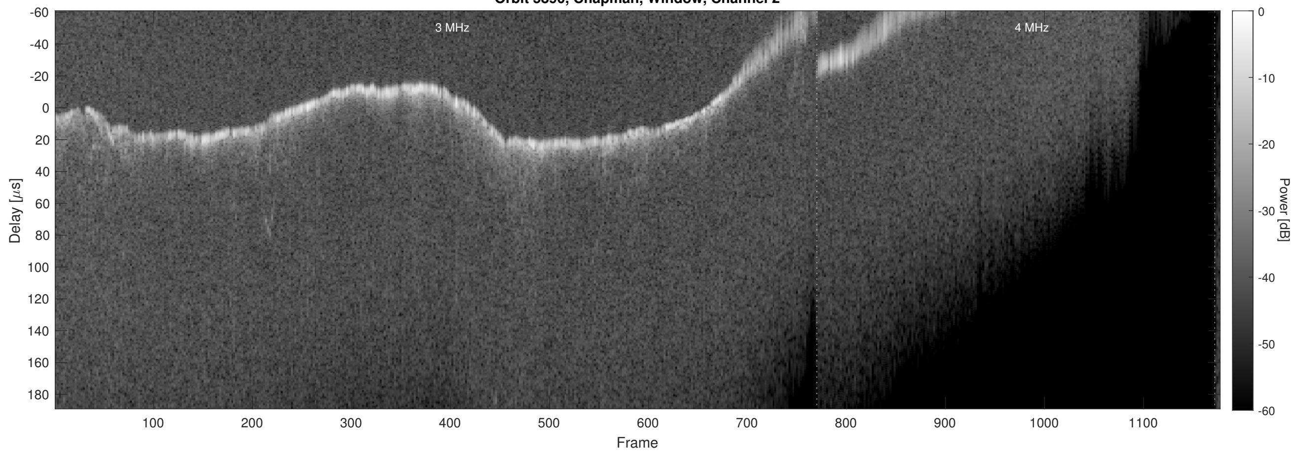
Orbit 5890, Chapman, Window, Channel 2
