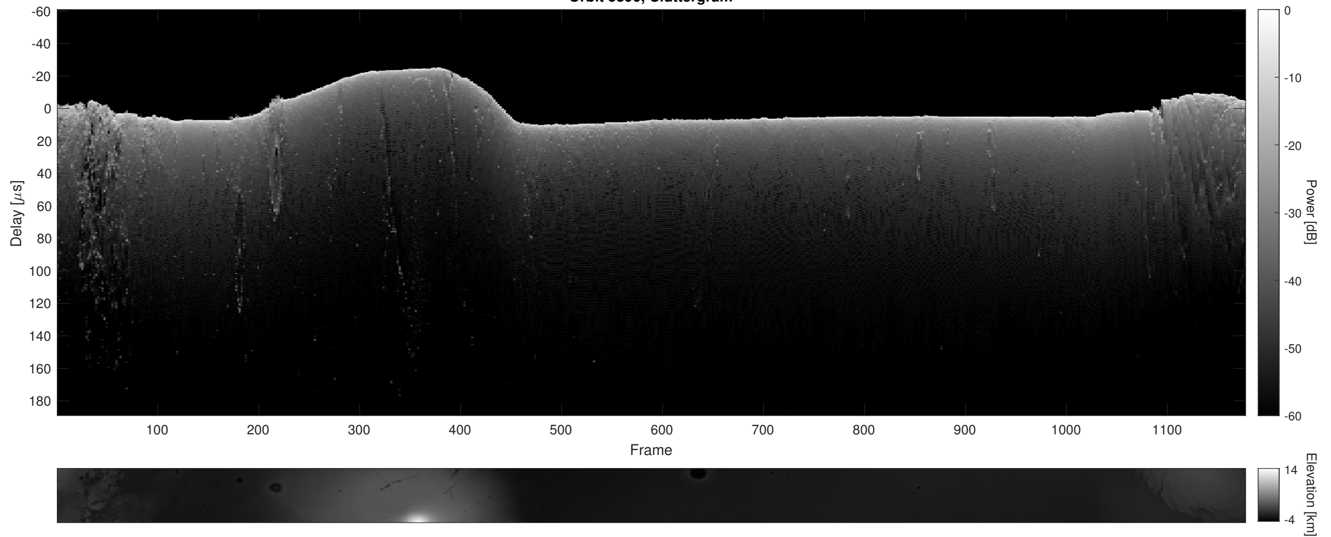
Orbit 5890, Cluttergram
