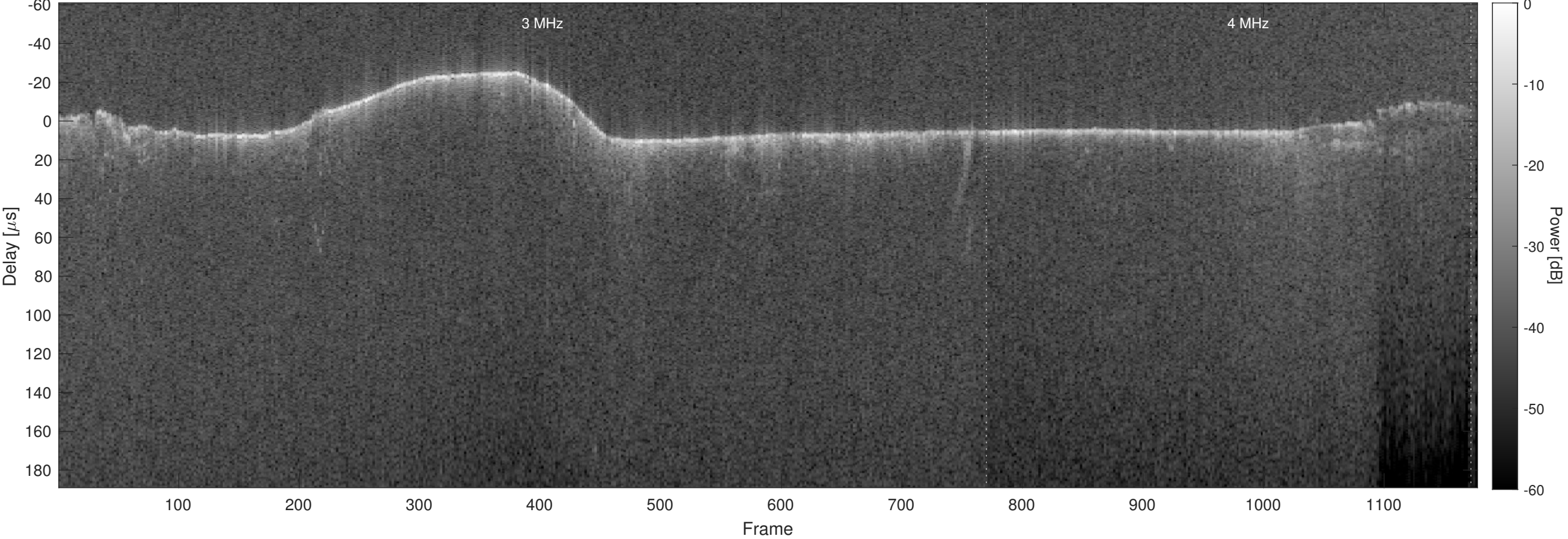
Orbit 5890, Optimized, No Window, Channel 2
