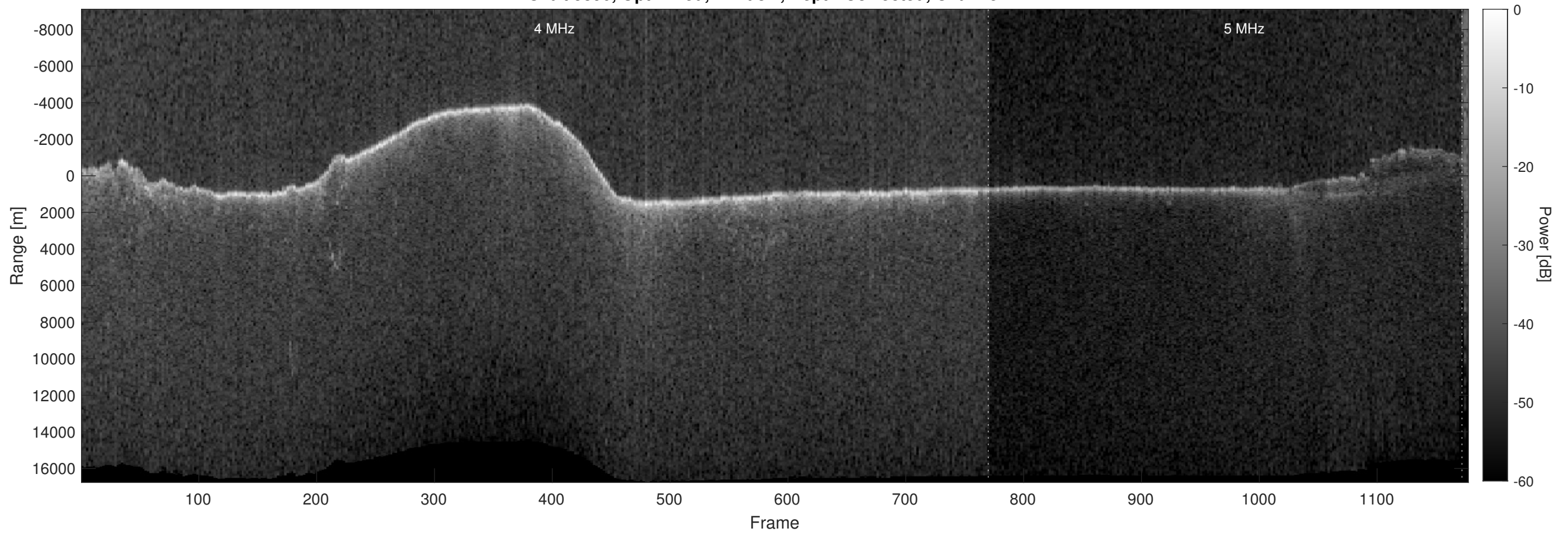
Orbit 5890, Optimized, Window, Depth-Corrected, Channel 2
