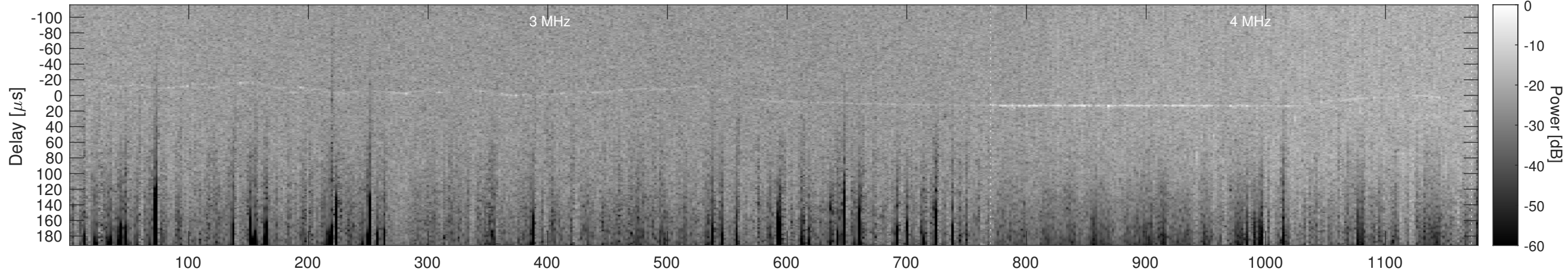
Orbit 5891, Cluttergram
