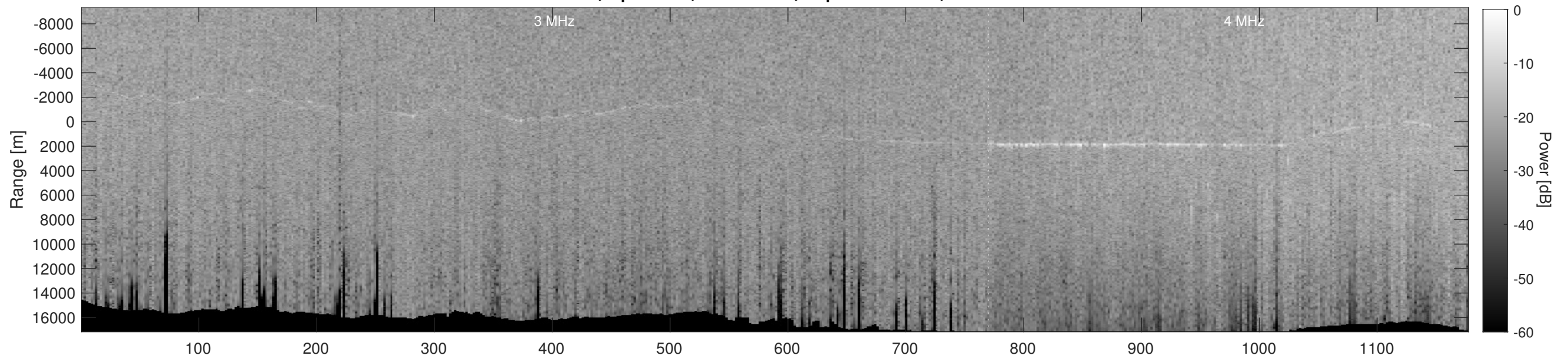
Orbit 5891, Depth-Corrected Cluttergram
