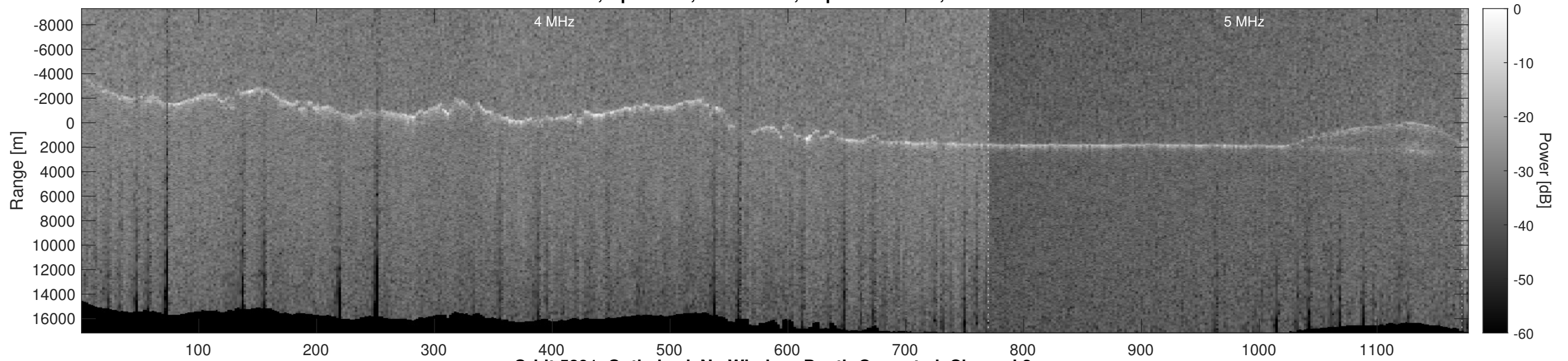
Orbit 5891, Optimized, No Window, Depth-Corrected, Channel 2
