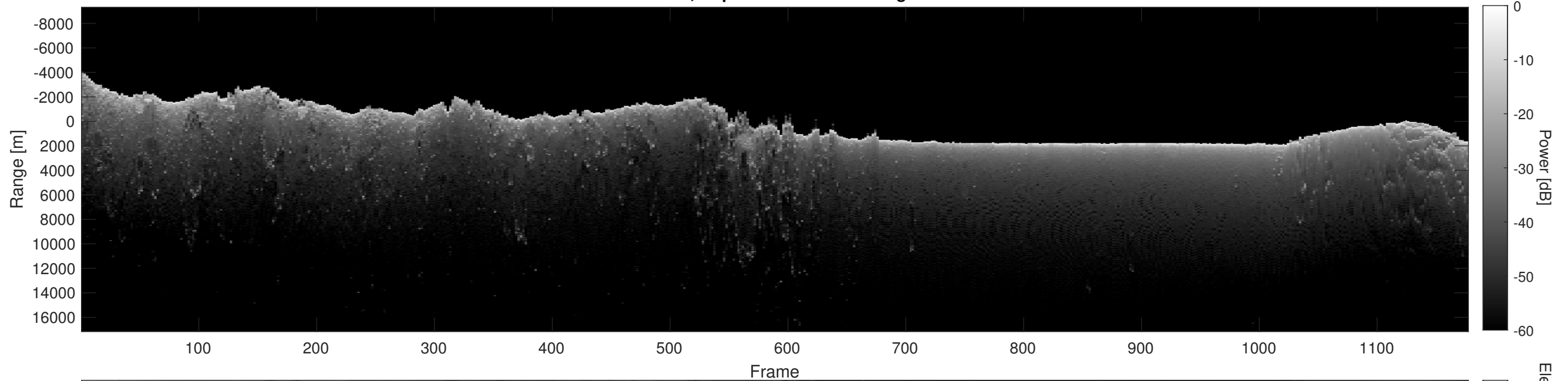
Orbit 5891, Depth-Corrected Cluttergram
