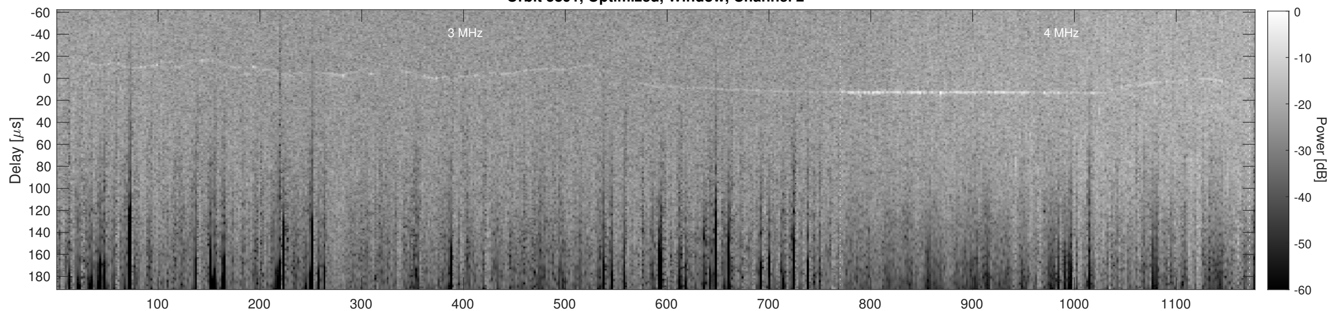
Orbit 5891, Cluttergram
