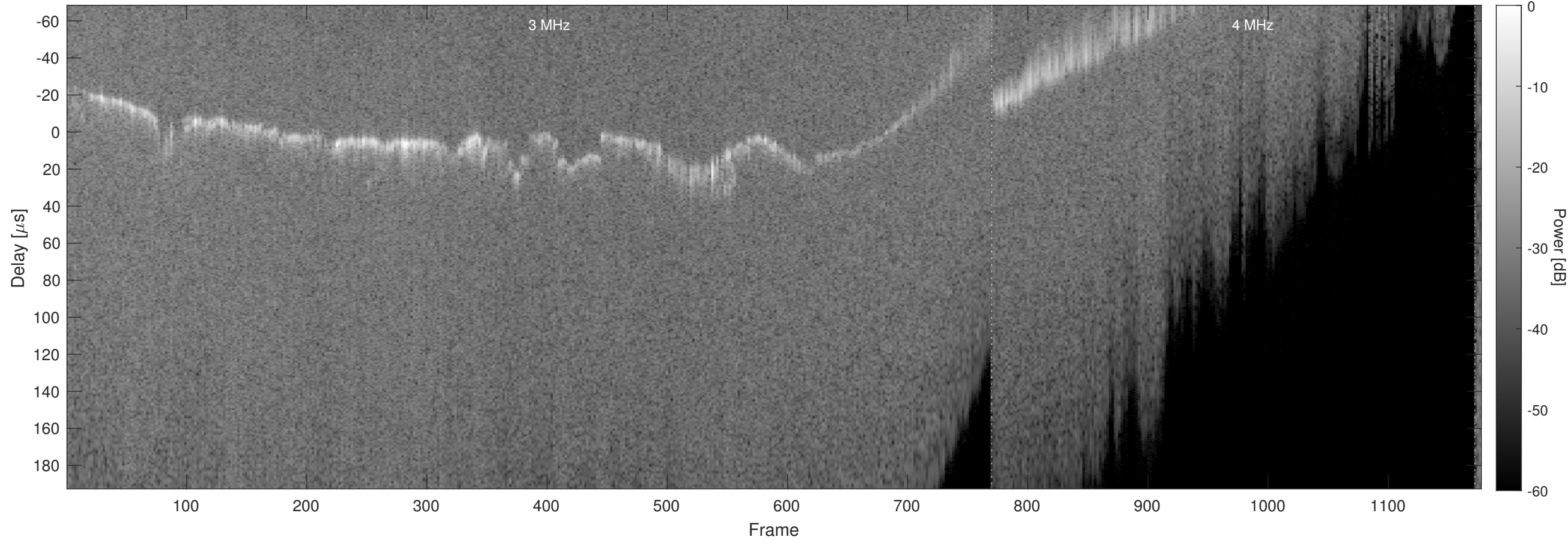
Orbit 5892, Chapman, No Window, Channel 2
