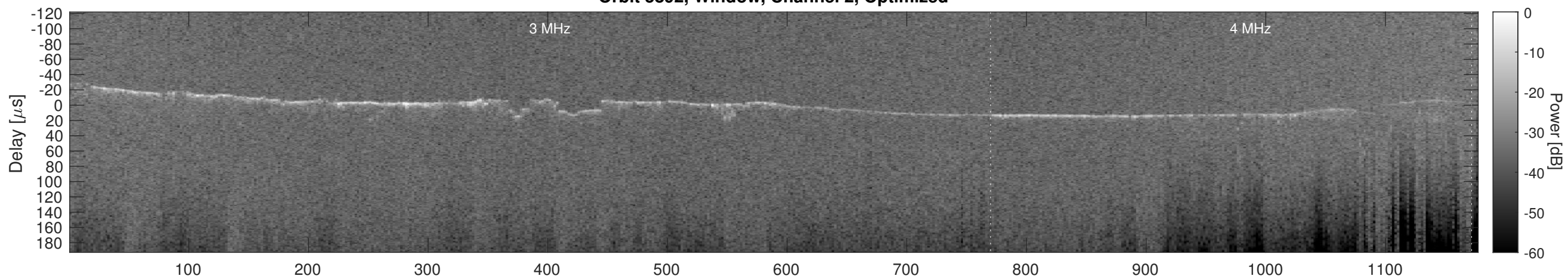
Orbit 5892, Cluttergram
