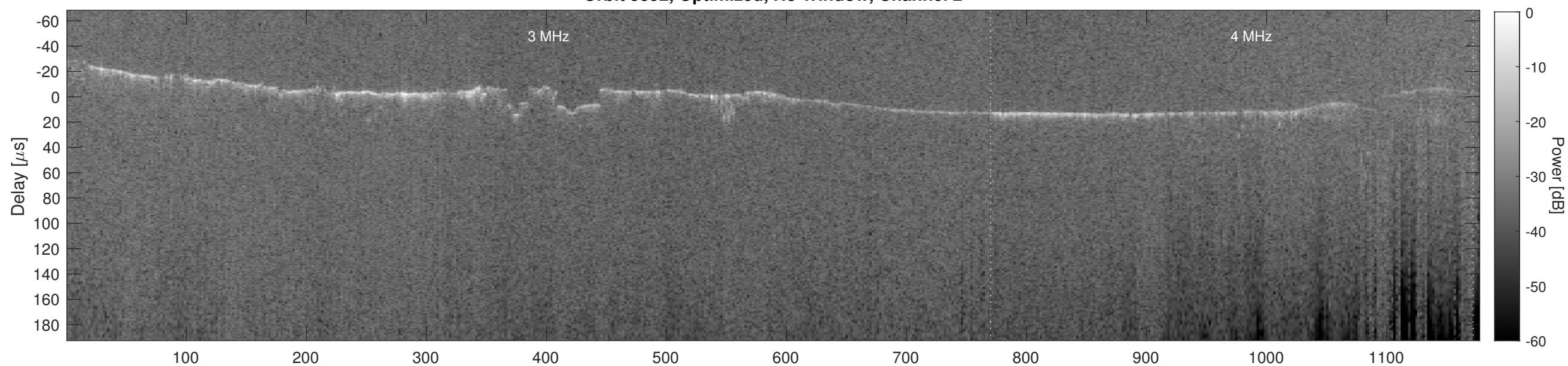
Orbit 5892, Cluttergram
