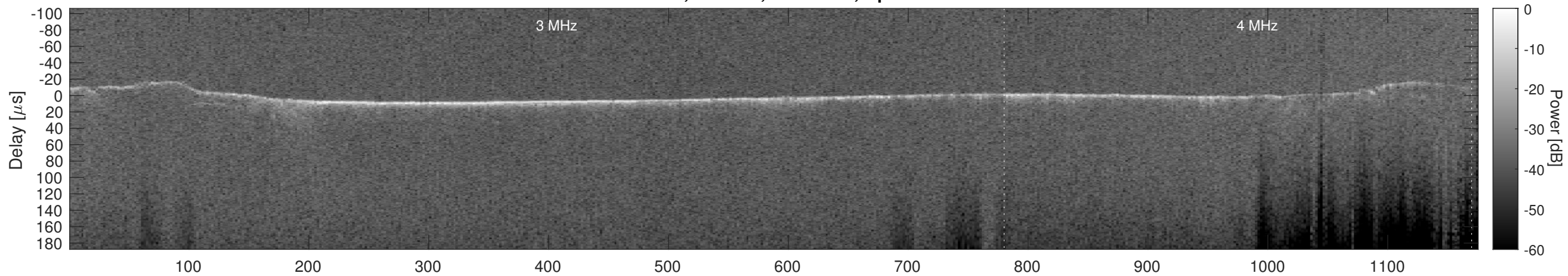
Orbit 5893, Cluttergram
