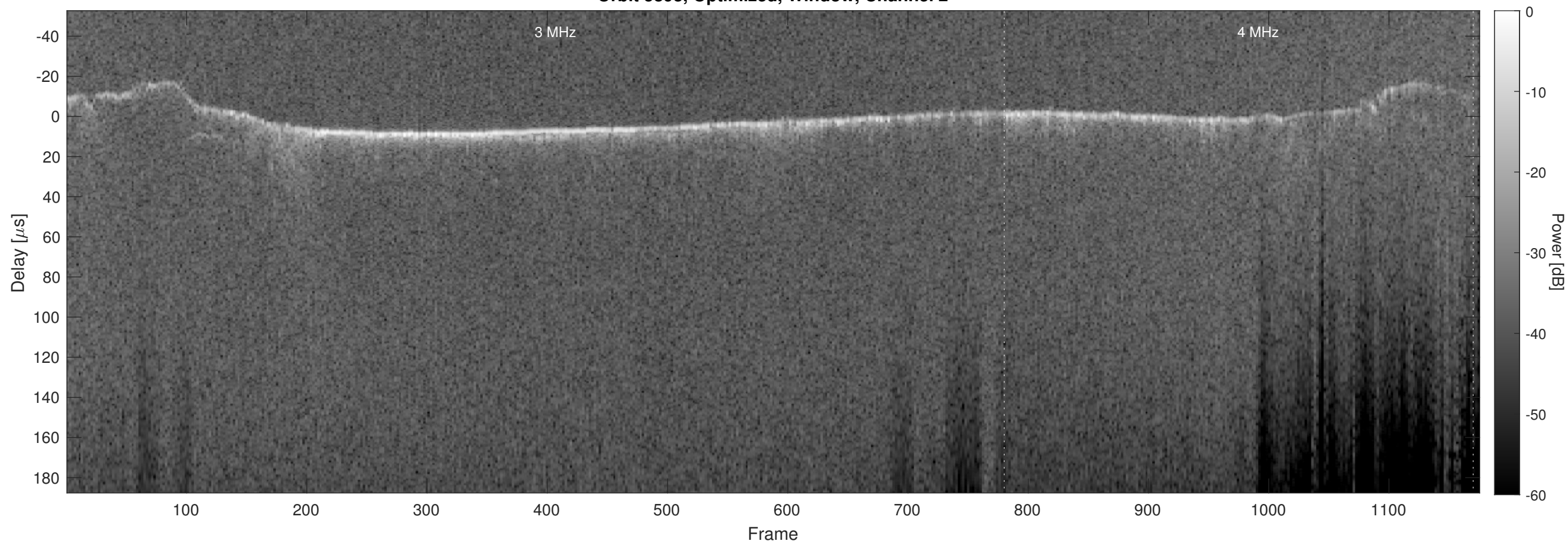
Orbit 5893, Optimized, Window, Channel 2
