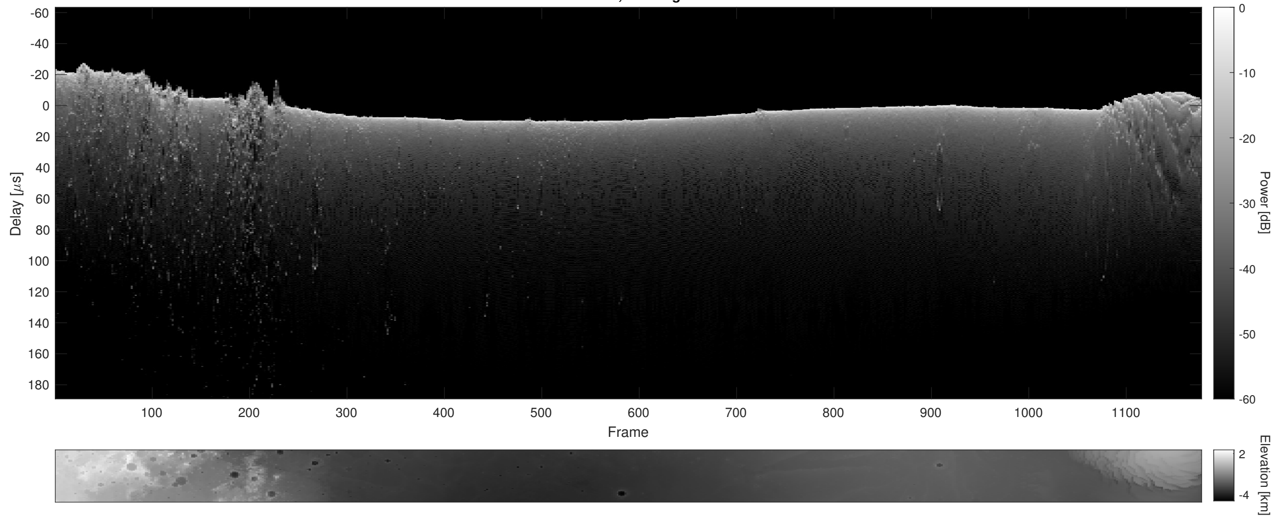
Orbit 5894, Cluttergram
