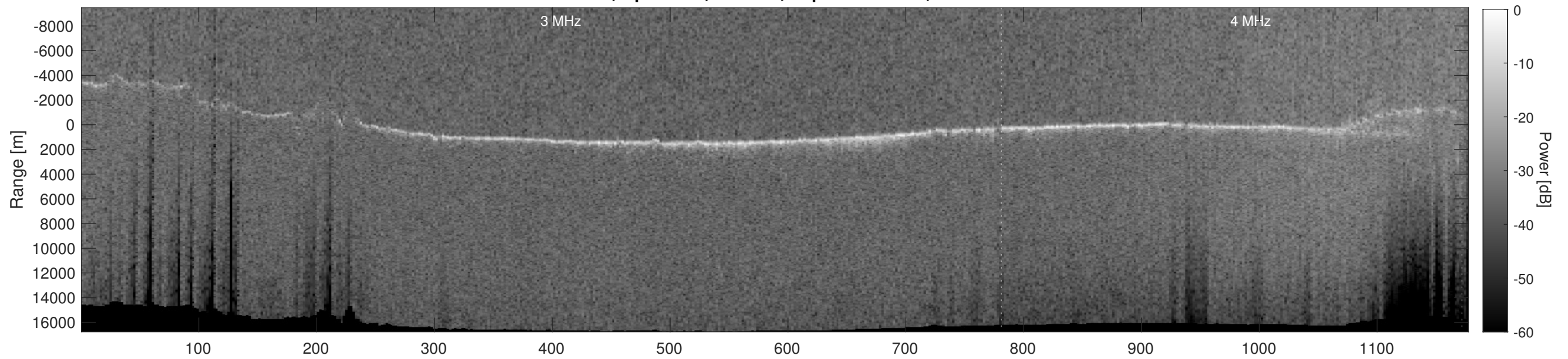
Orbit 5894, Depth-Corrected Cluttergram
