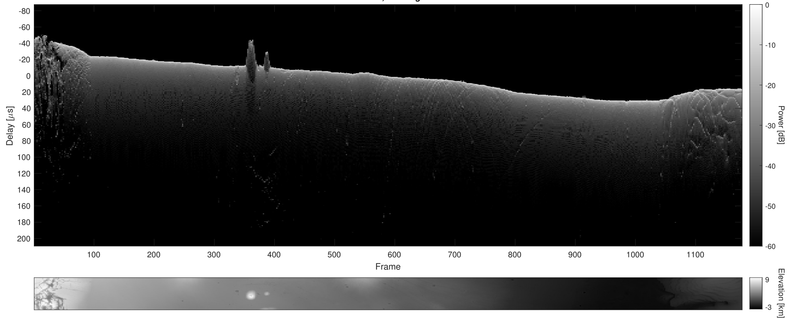
Orbit 5896, Cluttergram
