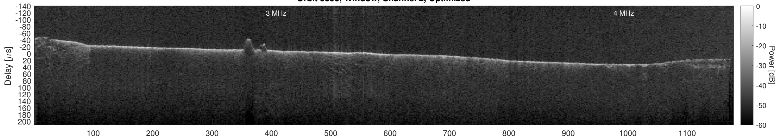
Orbit 5896, Cluttergram
