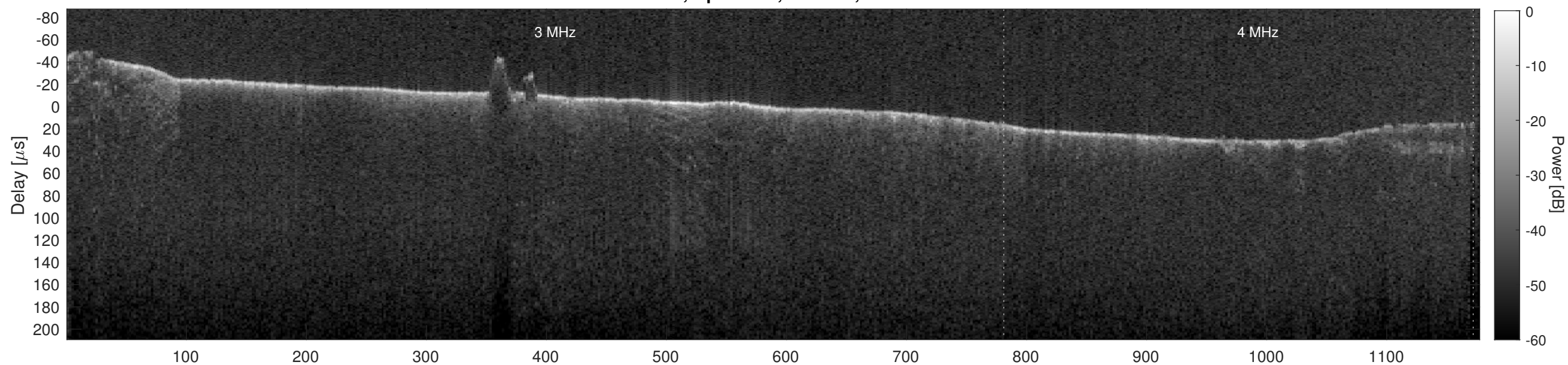
Orbit 5896, Cluttergram
