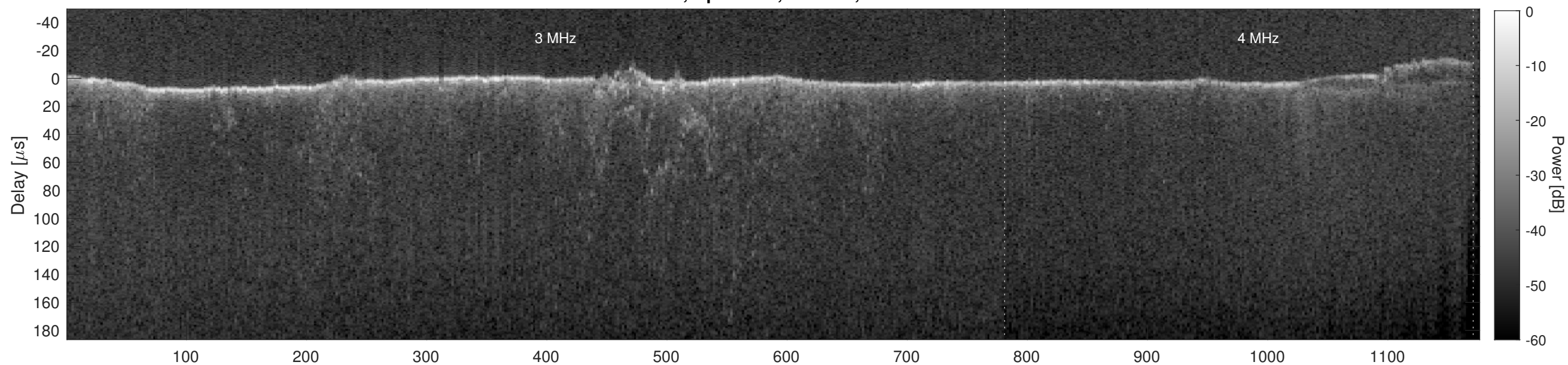
Orbit 5897, Cluttergram
