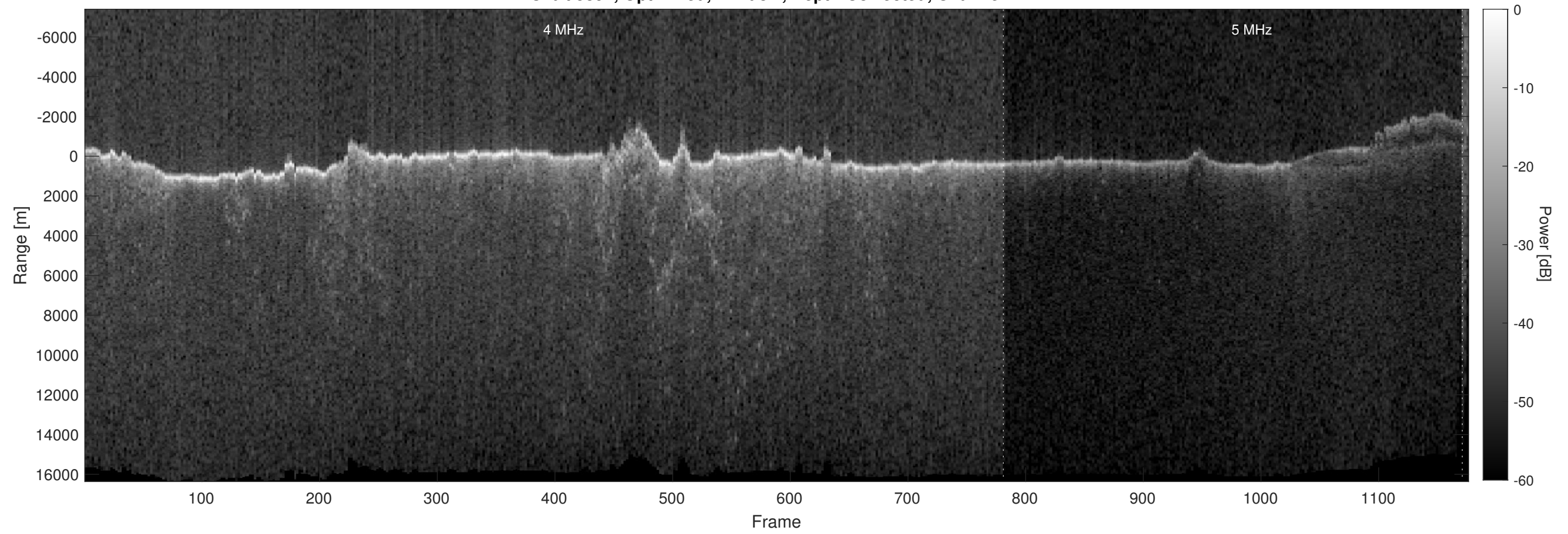
Orbit 5897, Optimized, Window, Depth-Corrected, Channel 2
