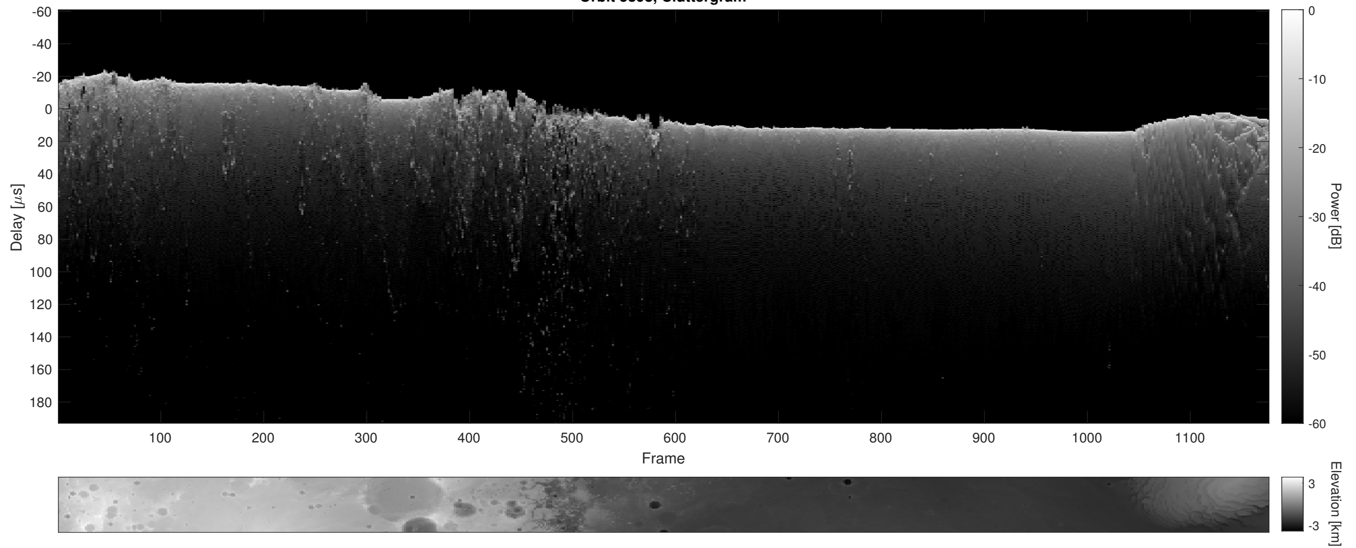
Orbit 5898, Cluttergram
